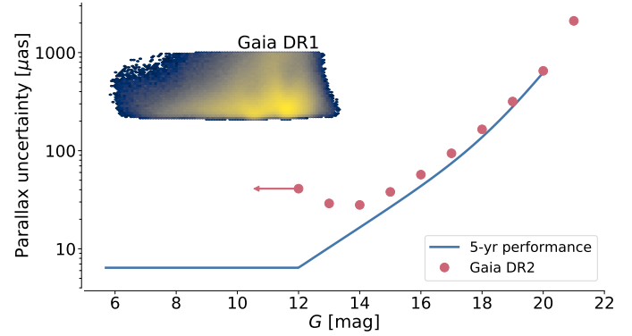
Fig. 7. Parallax uncertainties in Gaia DR2 (dots) as a function of G compared to the uncertainties quoted for Gaia DR1 (colour scale) and the expected end-of-mission parallax performance (solid line), as predicted after the commissioning of Gaia . Note how the performance for Gaia DR2 is still limited by calibration uncertainties for sources brighter than G \sim 14 .
